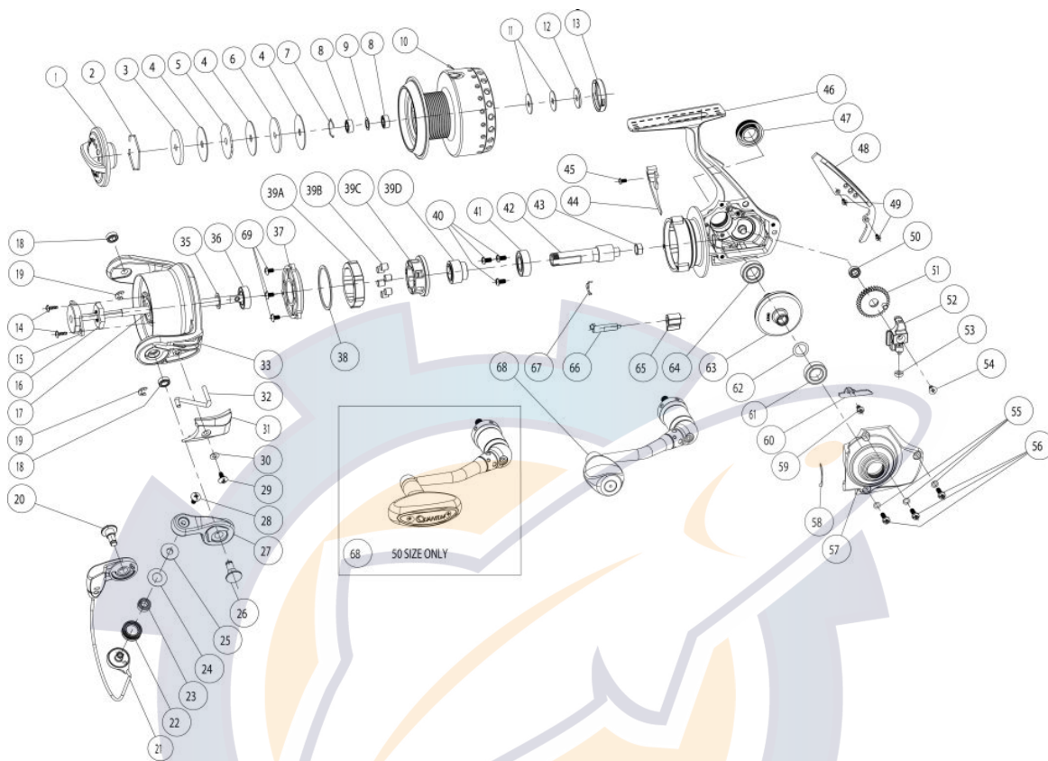
Quantum Energy EI40PTsB Spinning Reel Part List
